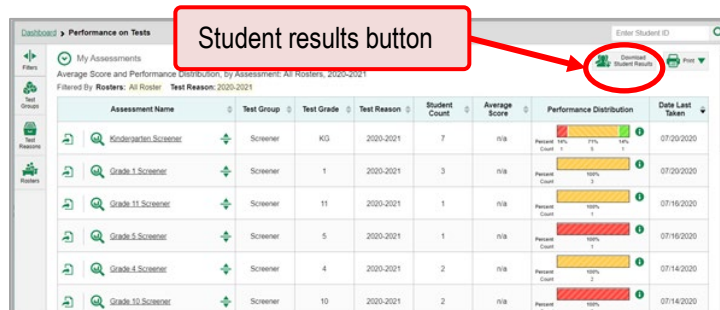
Figure 16. Dashboard
