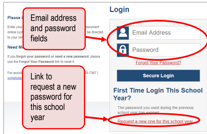
Figure 3. Login Page
