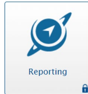
Figure 2. Reporting Card
